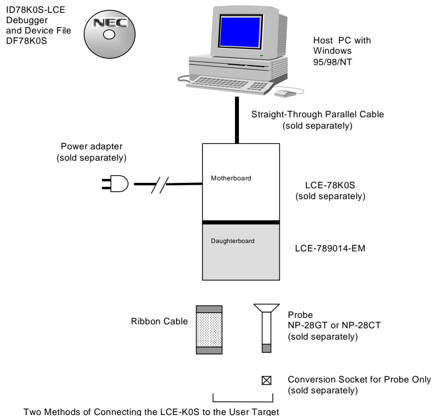
Two Methods of Connecting the LCE-K0S to the User Target
