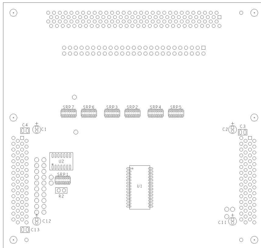
Figure 2. Top View of Daughterboard
